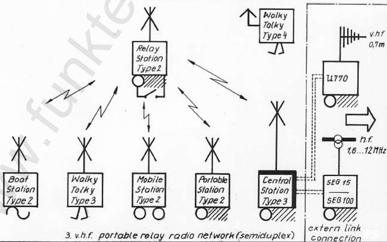
2. v.h.f. standard relay (semiduplex) radio network
